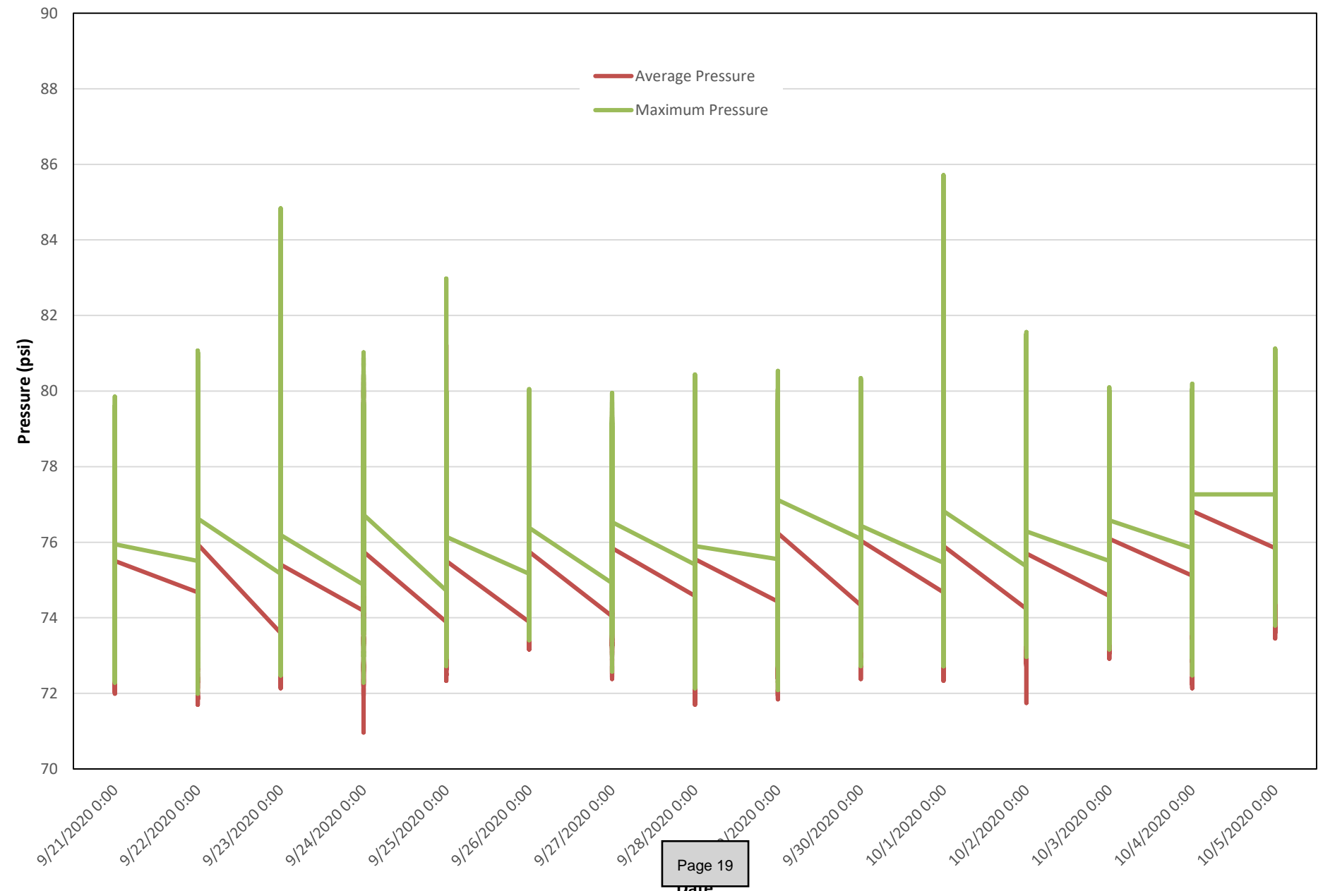
108 Crossing Way Pressure Readings
